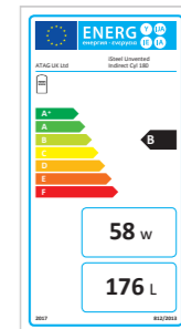
iSteel unvented 180l cylinder.
